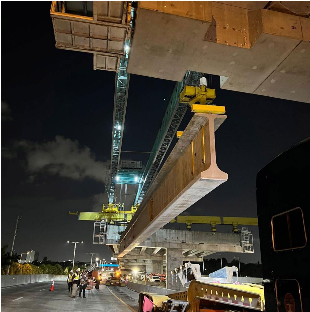
Erection of bridge beam for the new double-decked roadway on SR 836 over NW 17 Avenue
