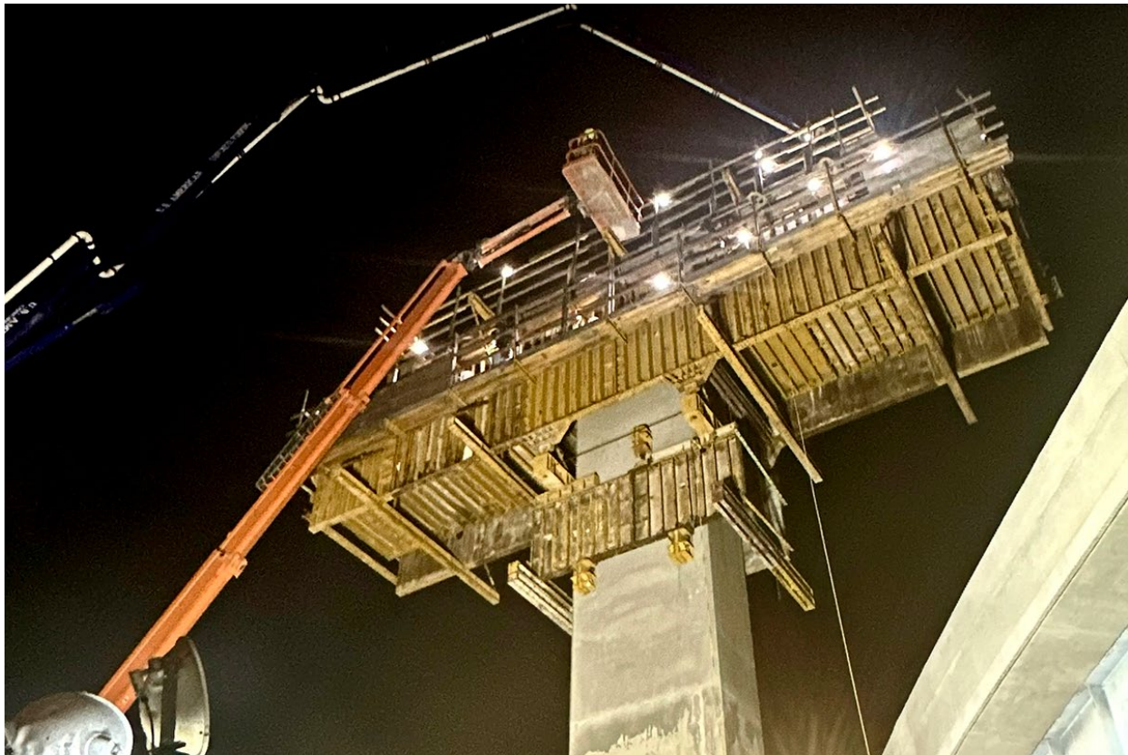
Pier cap concrete pour at the SR 836/I-95/I-395 interchange
